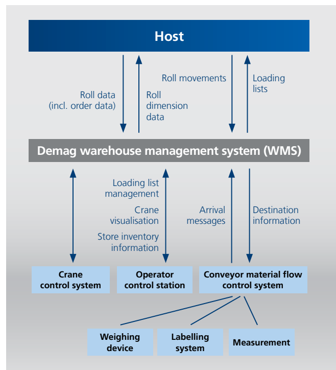
Interface to the Customer's host system: Demag Warehouse Management System
