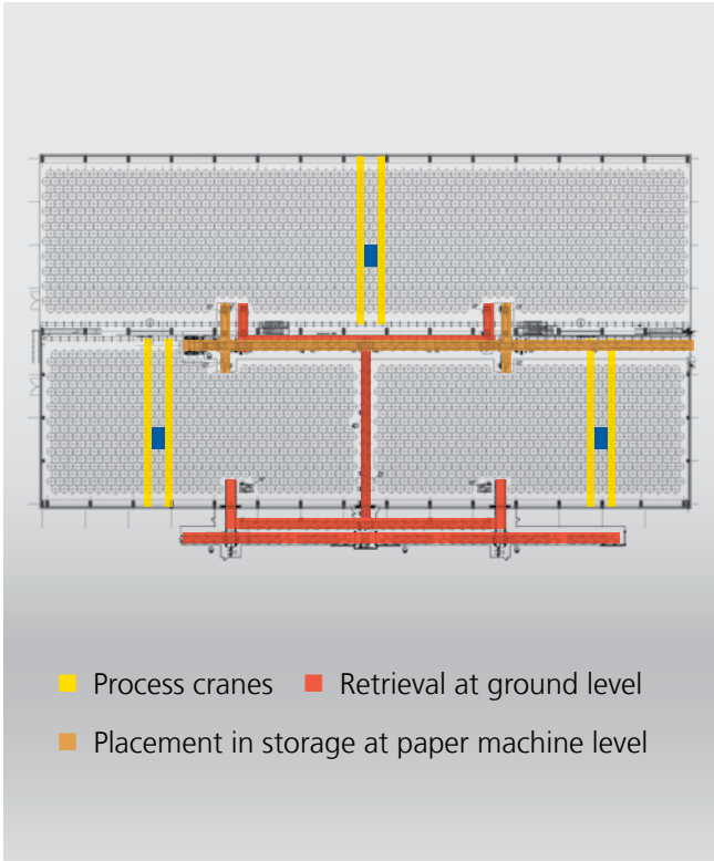
PM2 paper store installation layout
