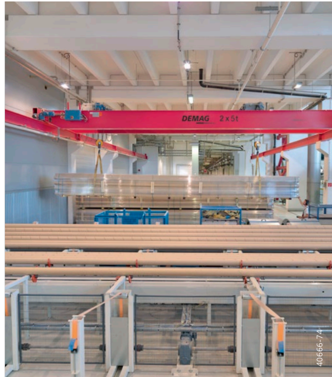
Demag double-girder overhead travelling crane with two hoists handles core packages
