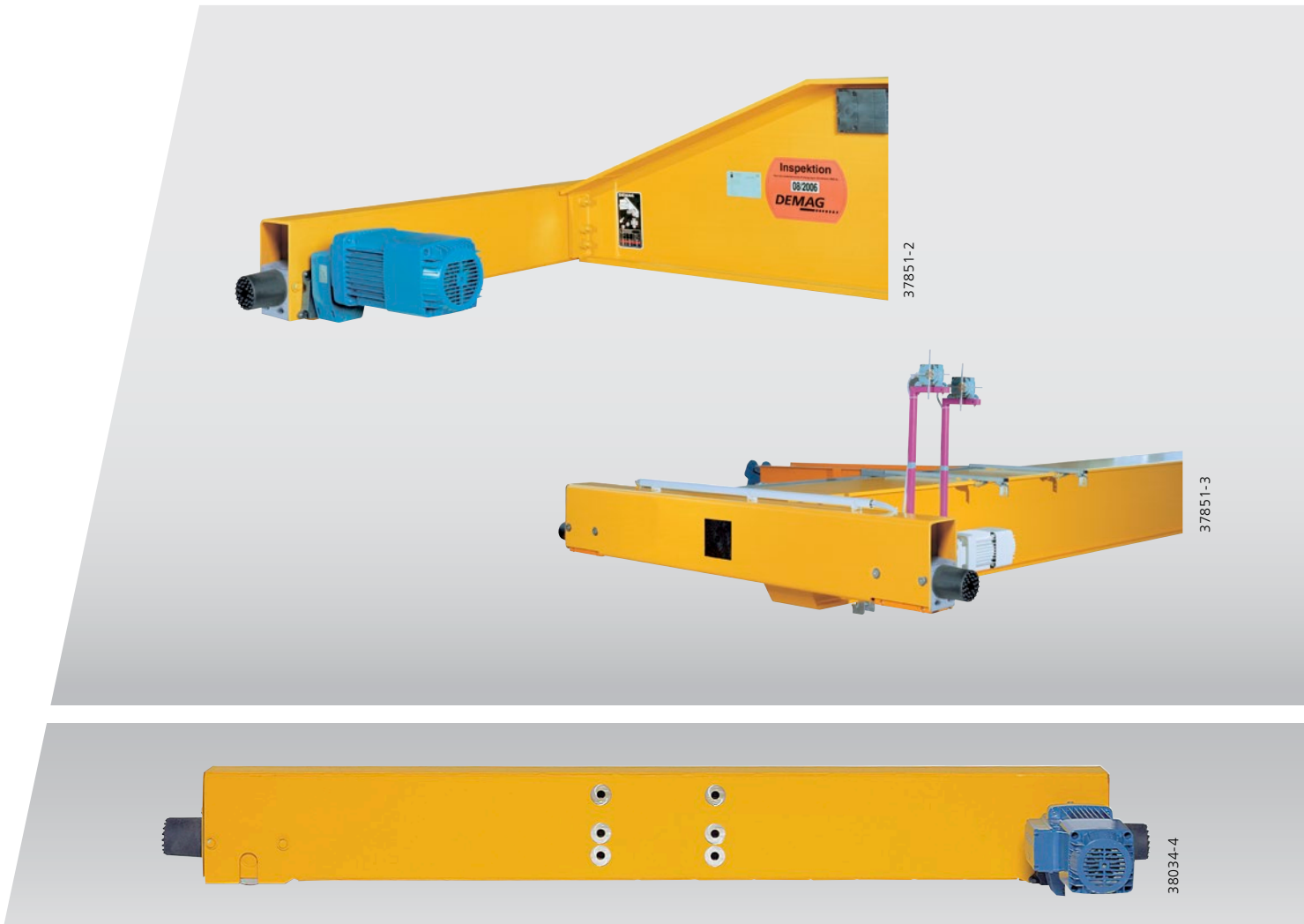
Crane end carriage with drive unit (A-type gearbox and Z-type motor) and Demag DPZ cellular foam buffer
