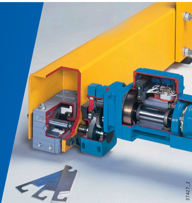
Travel units with spacer elements for track gauge adjustment
